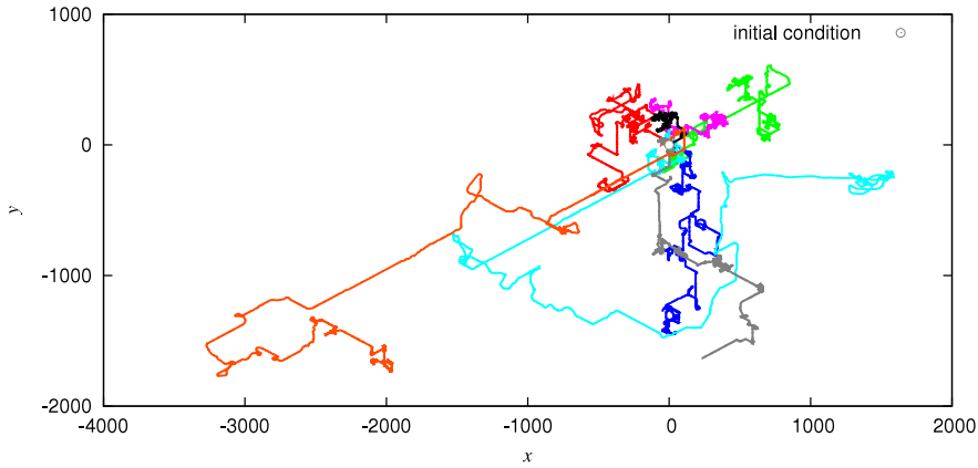
Figure 4. The trajectories of the centres of mass of benzene molecules starting from identical initial conditions for the centre of mass but different initial conditions for the internal degrees of freedom. The initial condition is (x, y) = (0, 0) , (p_x, p_y) = (0, 0) . Distances are in au ( a_0 = 0.529 177 \text{ \AA} ). The motion on the substrate is diffusive, and, for sufficiently long trajectories, the diffusion appears to be normal. (This figure is in colour only in the electronic version)
