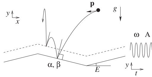
Figure 1. The bouncing-ball billiard with all its parameters. The horizontal motion on the periodic profile of the driving plate is formally similar to the motion of a particle on a substrate. The bouncing ball itself corresponds to the internal degrees of freedom of a molecule.
