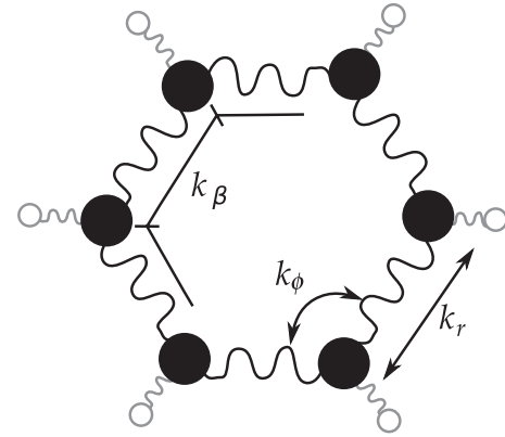
Figure 3. A schematic representation of the atomistic model for benzene. The hydrogen atoms and their bonds to the carbons are difficult to treat classically and have therefore been eliminated.
