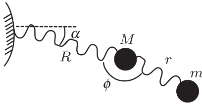
Figure 2. A simple atomistic model of a molecule with two atoms attached to a relatively heavy atom or group.
